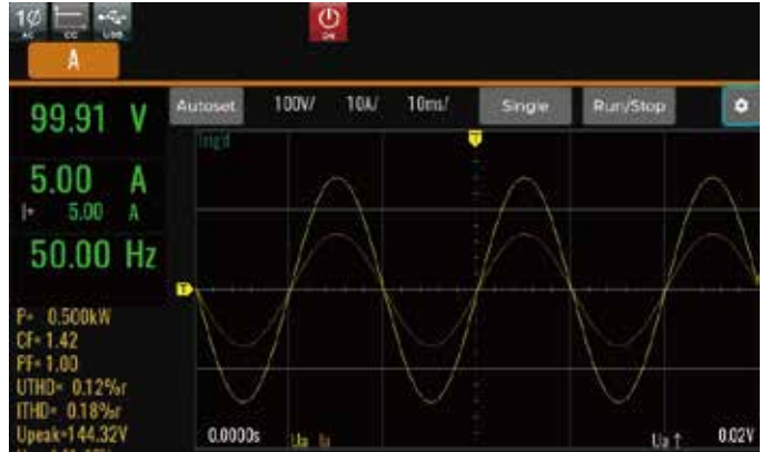
CC mode,CF=1.414
